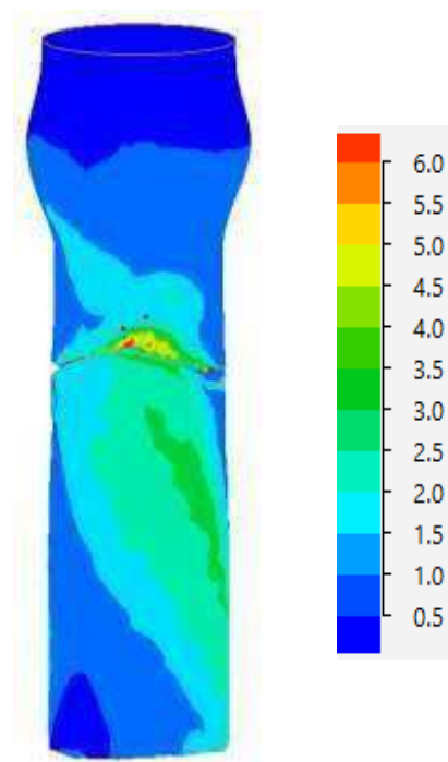
Fig. 3. Plastic deformation of the workpiece according to the SWP scheme
